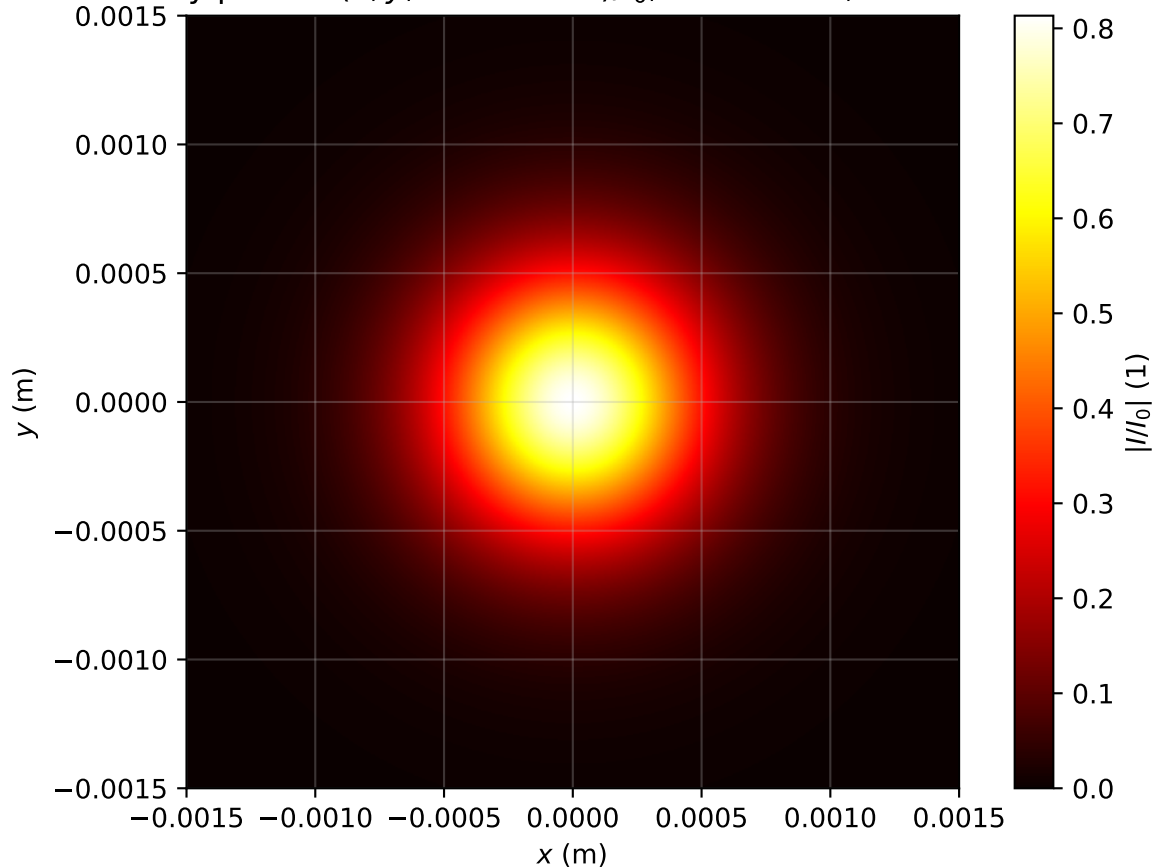
Intensity profile I(x, y, z = 2.468m)/I_0 , P_{in}=0.6P_{cr} , artificial time
